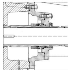
Single mech. seal, Design U unbalanced up to max. 16 bar
